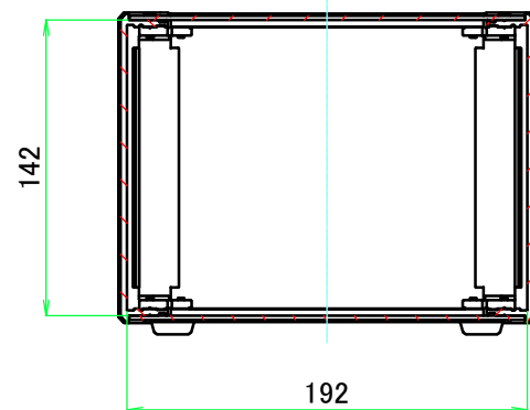
B-B (1:4)
