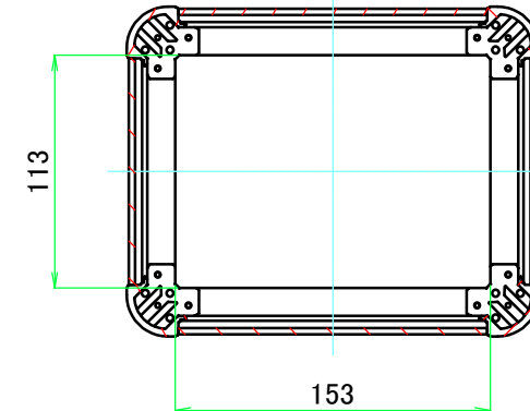
C-C (1:4)
