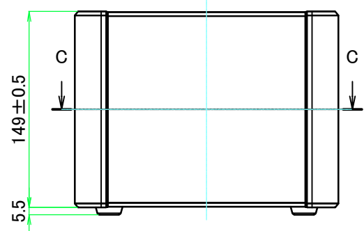
A view
